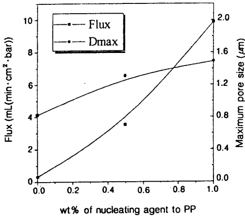
Figure 5. Performance change of hollow fiber membrane with different nucleating agent composition.
