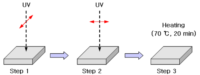
Figure 4. Experimental conditions for the LC alignment stability test.
