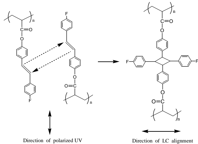
Figure 2. [2+2] cycloaddition reaction model of PVCN-F.
