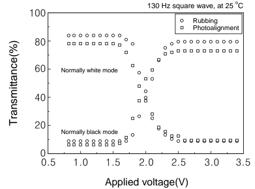
Figure 6. Electro-optical characteristics of twisted nematic LC cells.
